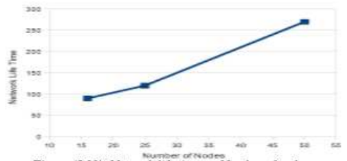
Figure (5-11): Network life time vs. Number of nodes.
