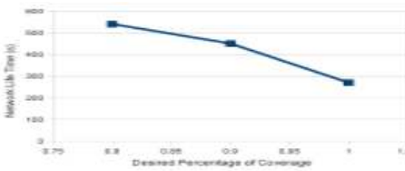
Figure (5-10) Network life time vs. desired coverage percentage for this 50 node network.
