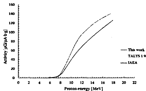
Fig. 1. The integral activity comparison for ^{186g}\text{Re}
